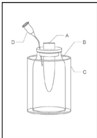
Figure (1): Drawing illustration of the collecting apparatus: (A) Root, (B) collecting glass vial, (C) Glass container, (D) Ventilating needle.
